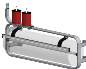
Dispenser attachment with cutter for 2 bobbins Ref.: 124221
