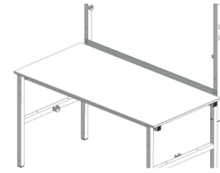
Backboard Ref. 700040
